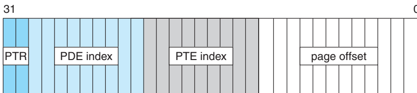
Figure 19.4 Virtual-to-physical address translation on IA-32.
