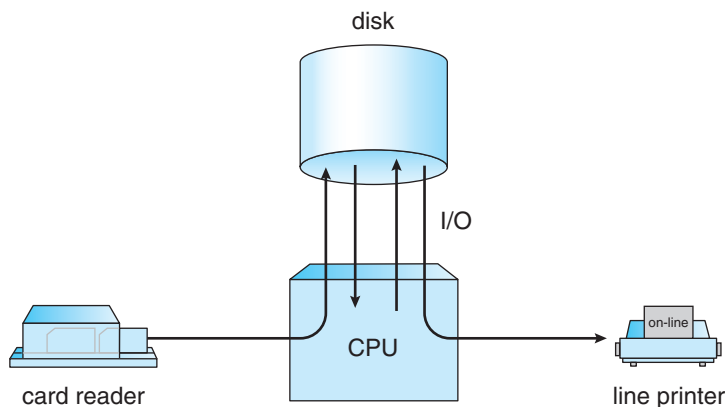
Figure 20.5 Spooling.
