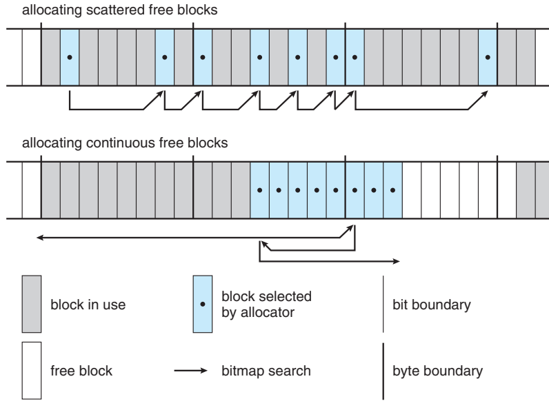
Figure 18.7 ext3 block-allocation policies.
