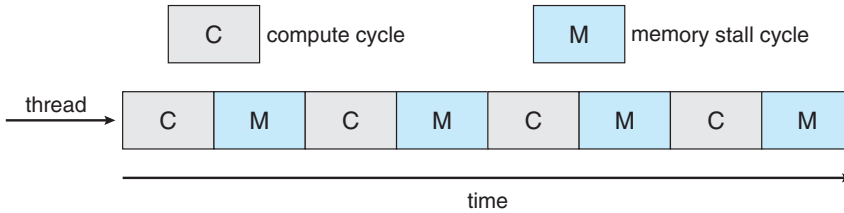
Figure 6.10 Memory stall.
