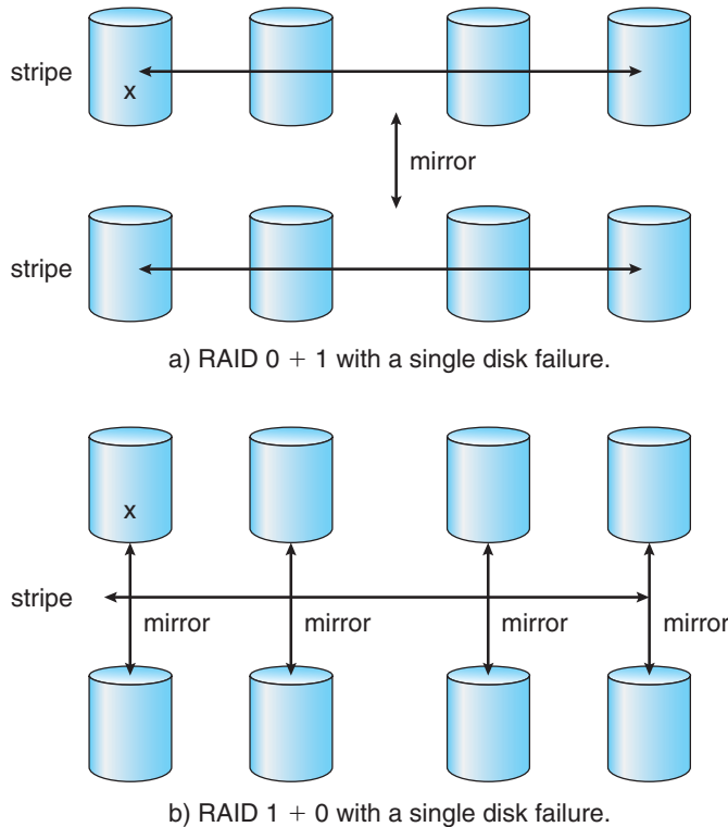
Figure 10.12 RAID 0 + 1 and 1 + 0.
