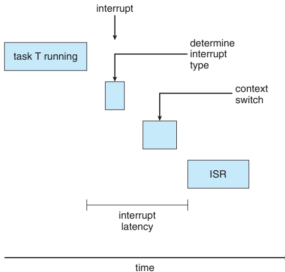
Figure 6.13 Interrupt latency.
