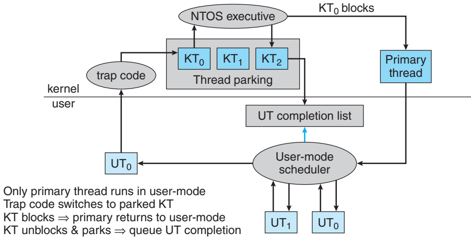
Figure 19.11 User-mode scheduling.
